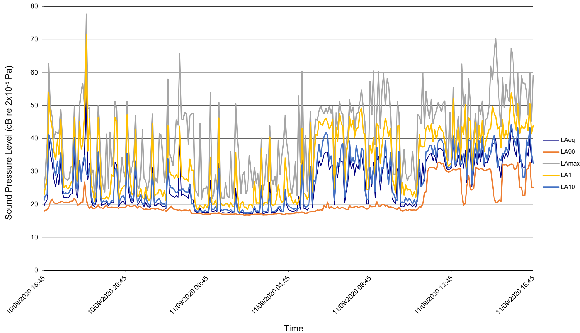
Monitoring Location 2 Internal Measured L_{Aeq} , L_{A90} , L_{AFmax} , L_{A1} , L_{A10} Time History
